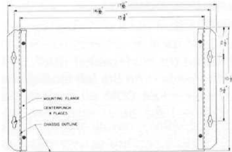
Fig. 4—Bottom of MC240 with mounting flanges attached.
